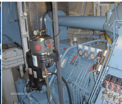
Scana Volda, 2000Kva, 1800 Kw, Lubricant: Mobilgear XP 600 100
